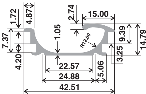
Section No. 1929 Wt. Range(kg/12') 1.250-1.400
