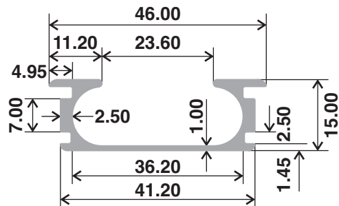
Section No. 1930 Wt. Range(kg/12') 1.450-1.650
