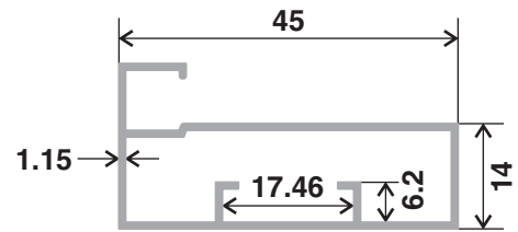
Section No. 1926 Wt. Range(kg/12') 1.550-1.750
