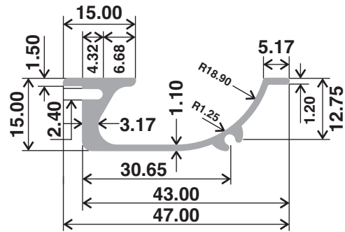
Section No. 1928 Wt. Range(kg/12') 1.350-1.450
