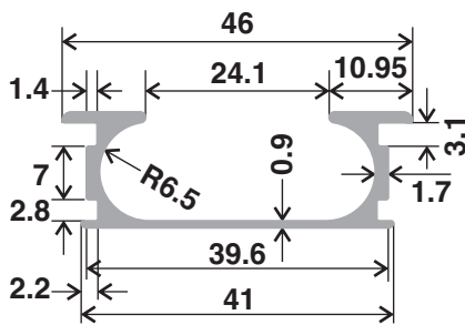
Section No. 1927 Wt. Range(kg/12') 1.250-1.350
