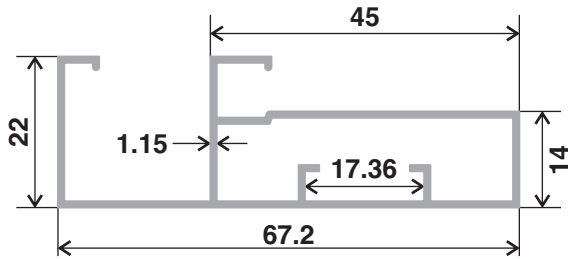
Section No. 1925 Wt. Range(kg/12') 1.950-2.150
