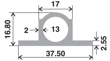
Section No. Wt. Range(kg/12') 2110 1.750-1.900
