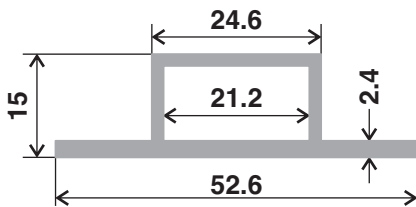
Section No. Wt. Range(kg/12') 2130 1.950-2.100
