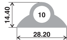
Section No. Wt. Range(kg/12') 2140 1.700-1.850
